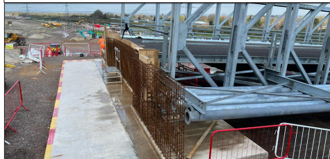
Bailey Bridge retaining wall
